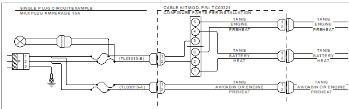
B.1. Example of single plug circuit using Cable Kit Mod p/n: TC03321/TAC03321. Refer to Drawing: 03320 and Appendix § D Table D.5.
