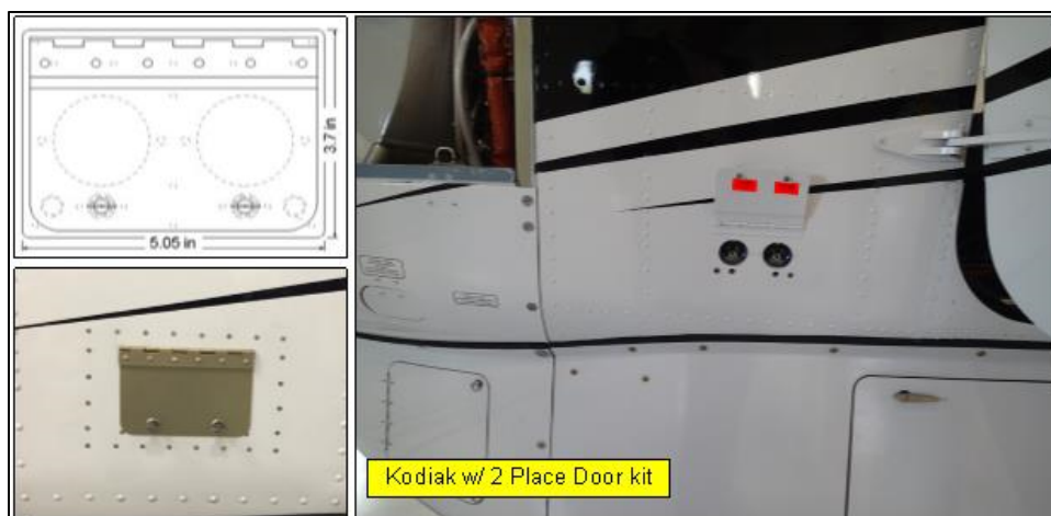
A.15. Example of 2-Place Plug Door Kit p/n: TD03152/TAD03152 located in sheet metal panel. Single plug door kits and cabling options available, refer to Appendix §§ B and D.
