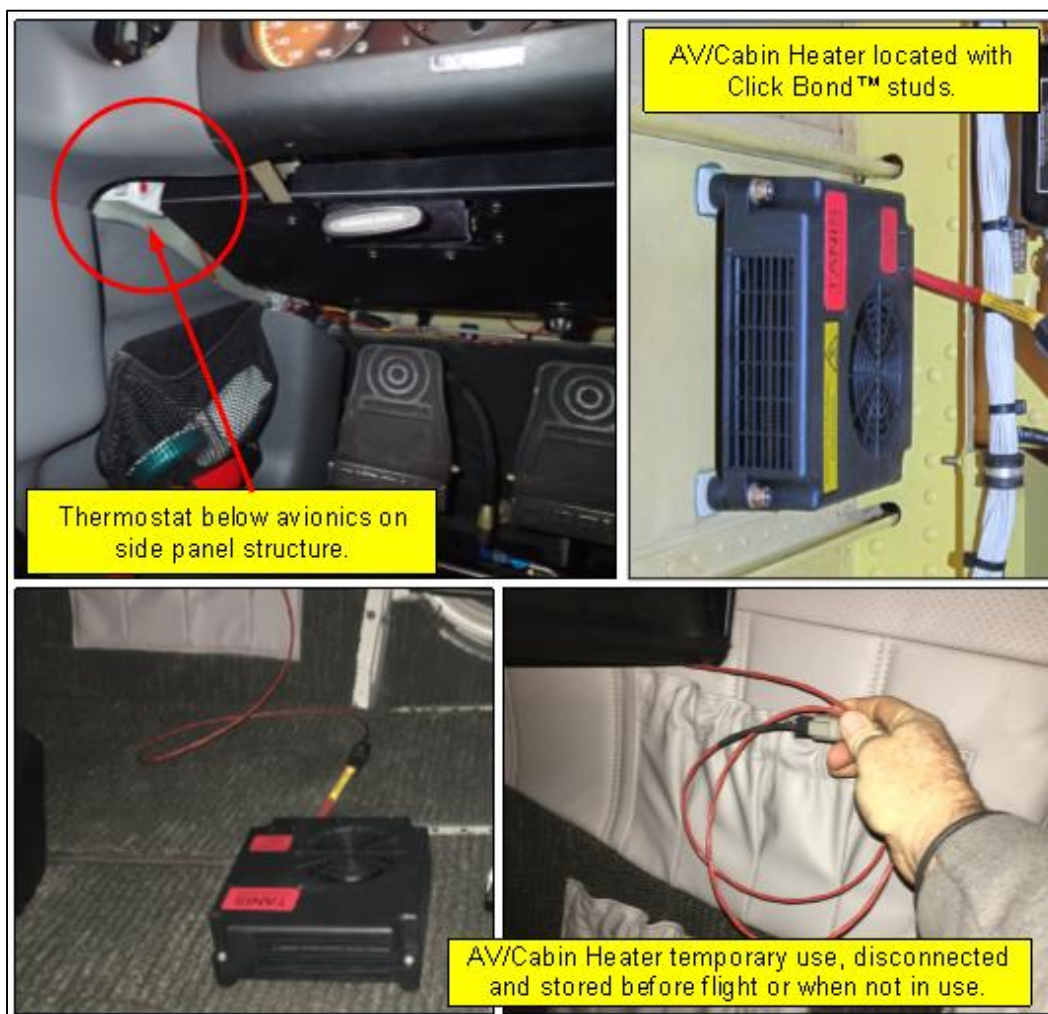
Figure 9.11. Example of AV/Cabin Heat Kit p/n: TU03323/TAU03323. The kit may be configured for occasional use or permanently installed. The heater is also available individually for occasional use as a space heater. For standard options refer to Appendix §§ B and D.
